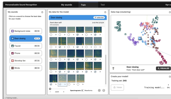
Figure 1: Overview of the SPECTRA pipeline. In an interactive machine learning training workflow, users collect audio data samples (left), filter their data into a training dataset (center), and assess their model’s performance in a live environment (right). The design includes key elements to support the needs of DHH users during this process, including spectrogram and waveform audio visualizations of audio, data annotating to save useful contextual information, and an interactive clustering visualization of their dataset.
