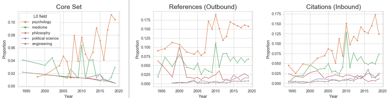
Figure 4: Proportions of non-CS fields represented among papers in the core set over time (left), and among the papers referenced by (center) and citing (right) papers in the core set. The proportions of papers on the topic of psychology, and medicine to a lesser degree, have increased over time, especially among citations. Only years with greater than 5 papers are shown.
