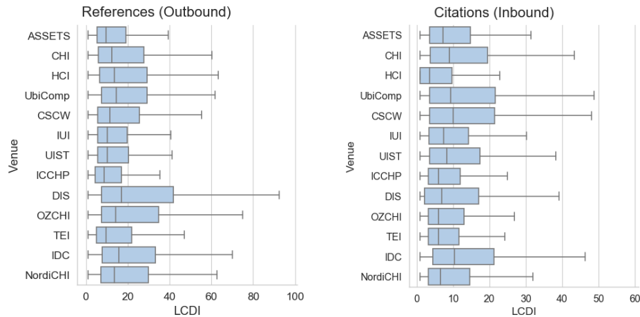
Figure 5: Distribution of the LCDI [15] computed over the L1 fields of study of referenced papers (left) and citing papers (right) for each of 13 venues in the comparative dataset. Higher LCDI indicates higher diversity among the fields of the references or citations. LCDI is similar across venues but is lower for those focused on a particular subdomain (e.g. ASSETS, IUI, ICCHP, TEI) or regional conferences (OZCHI, NordiCHI) and higher for more general HCI conferences (CHI, UbiComp).
