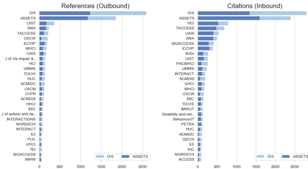
Figure 2: Top venues of papers referenced by (left) and citing (right) accessibility papers in the core set. References and citations are both dominated by papers from CHI and ASSETS, though a relatively larger proportion of citations arrive from other publication venues.
